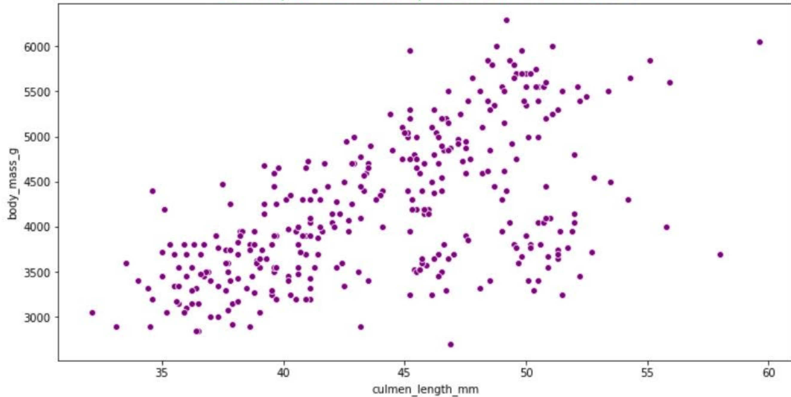
Scatterplot-Relationship between two variables
