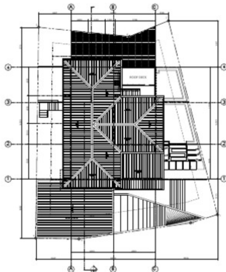
ROOF DECK PLAN
