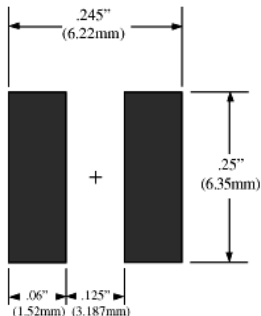
PC Board
