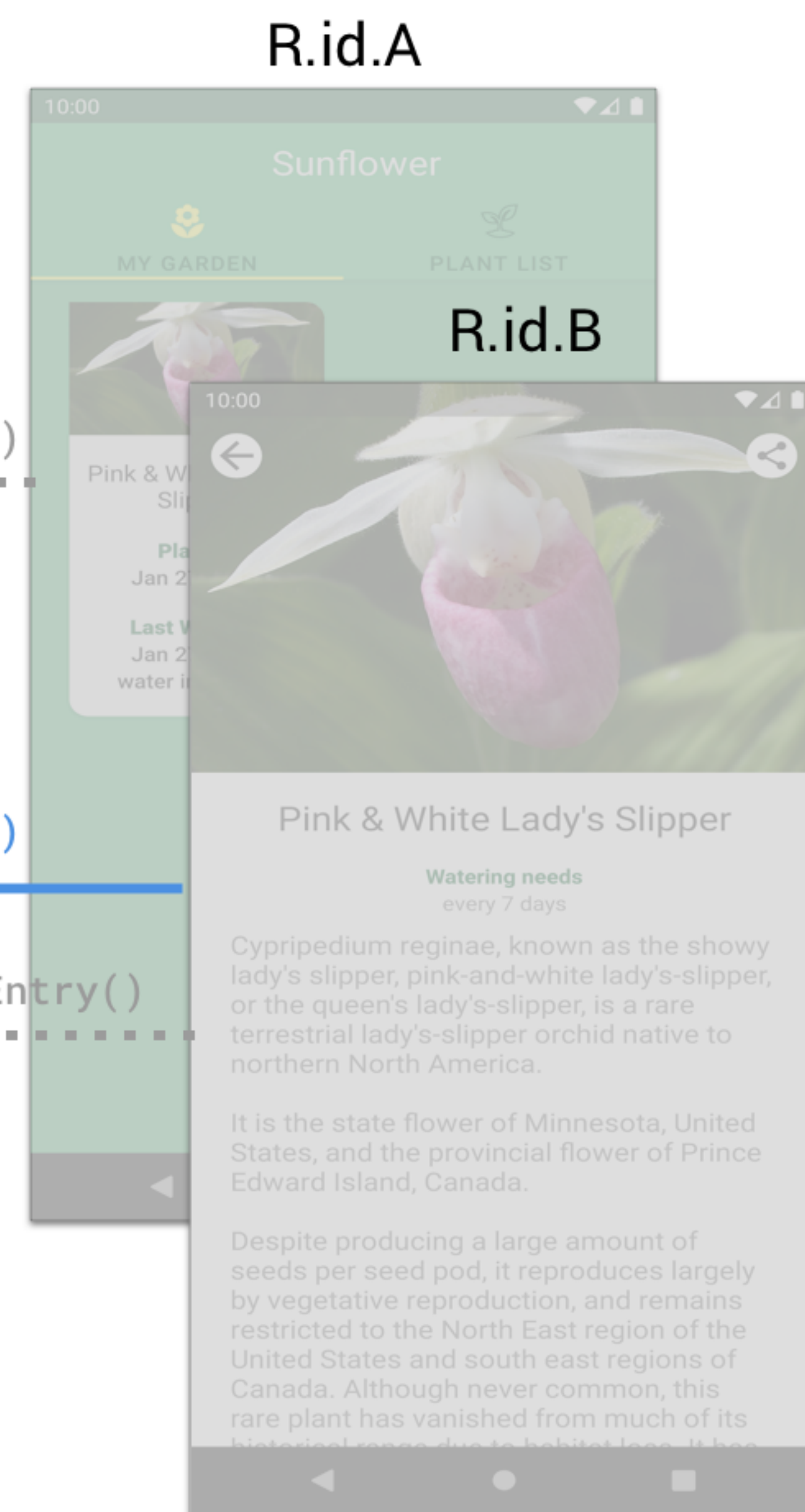
Navigation BackStack
