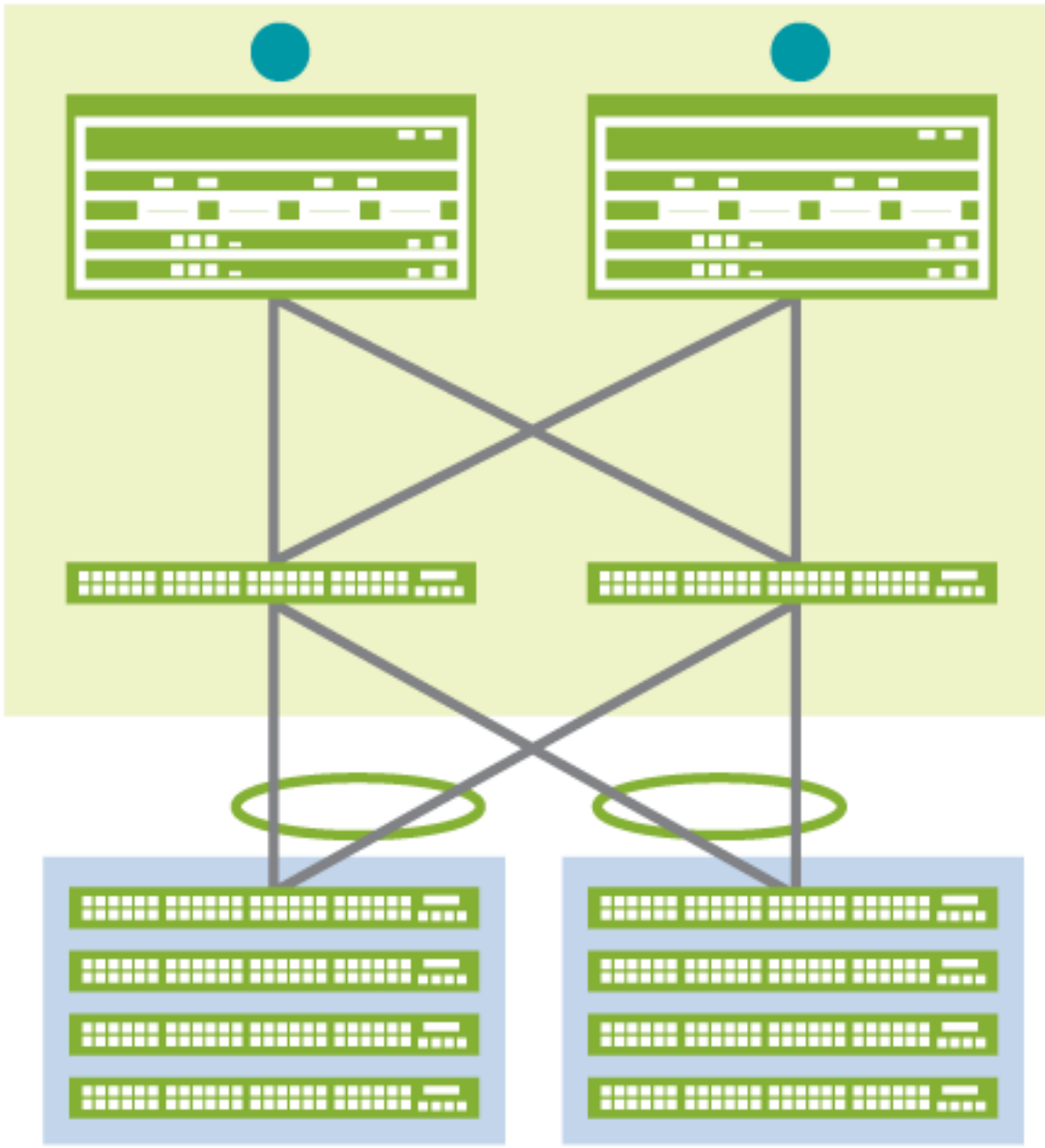
Campus Fabric Core-Distribution Centrally-routed Bridging
