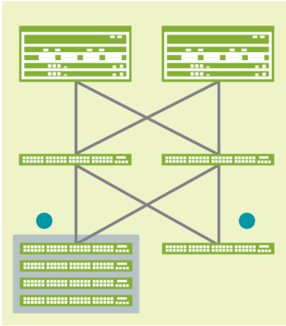
Campus Fabric IP Clos End-to-End
