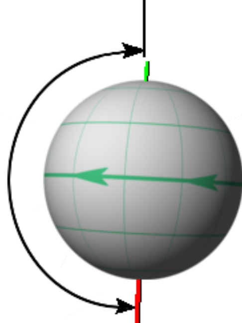
Venus: 177^\circ
