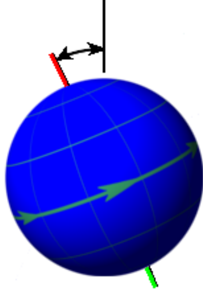
Earth: 23^\circ
