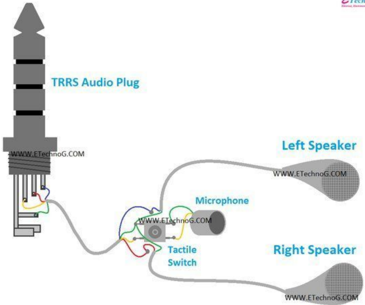
Stereo Headphone Jack Wiring and Connection Diagram
