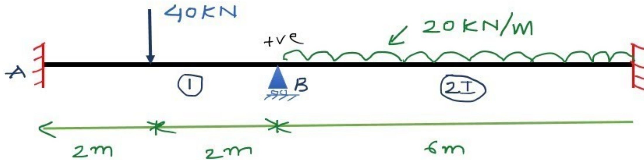
Two Span Continuous beam.
