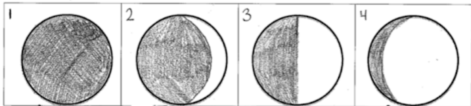
New Moon
