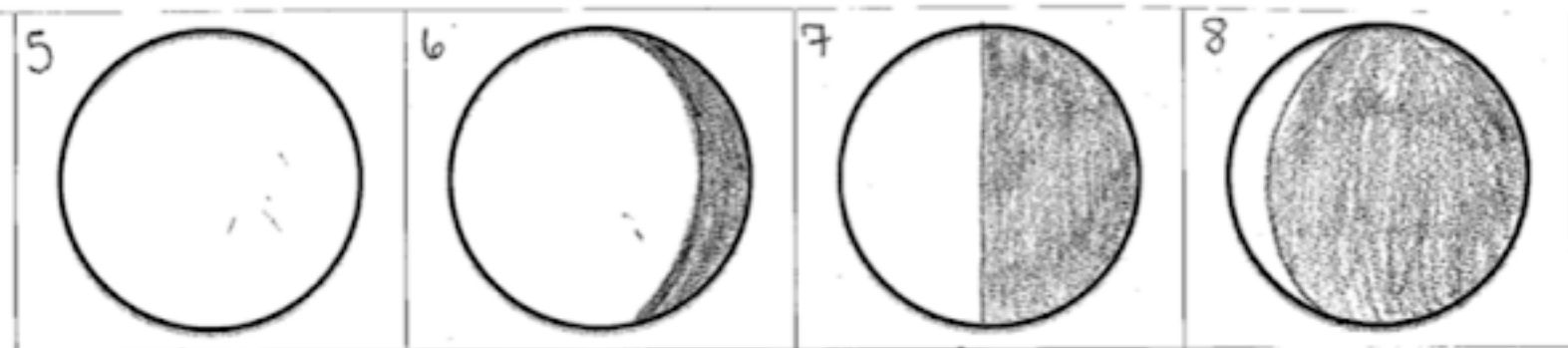
Full Moon
