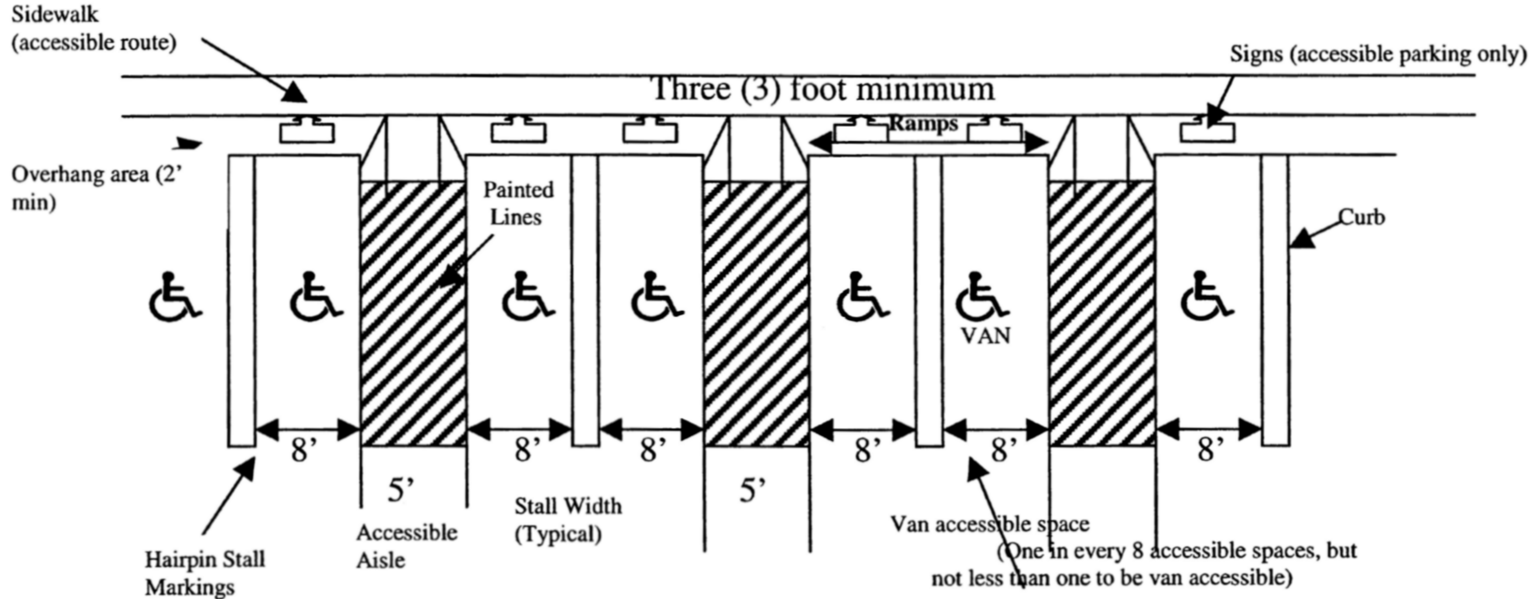
Figure 1—Accessible Parking Space Standards
