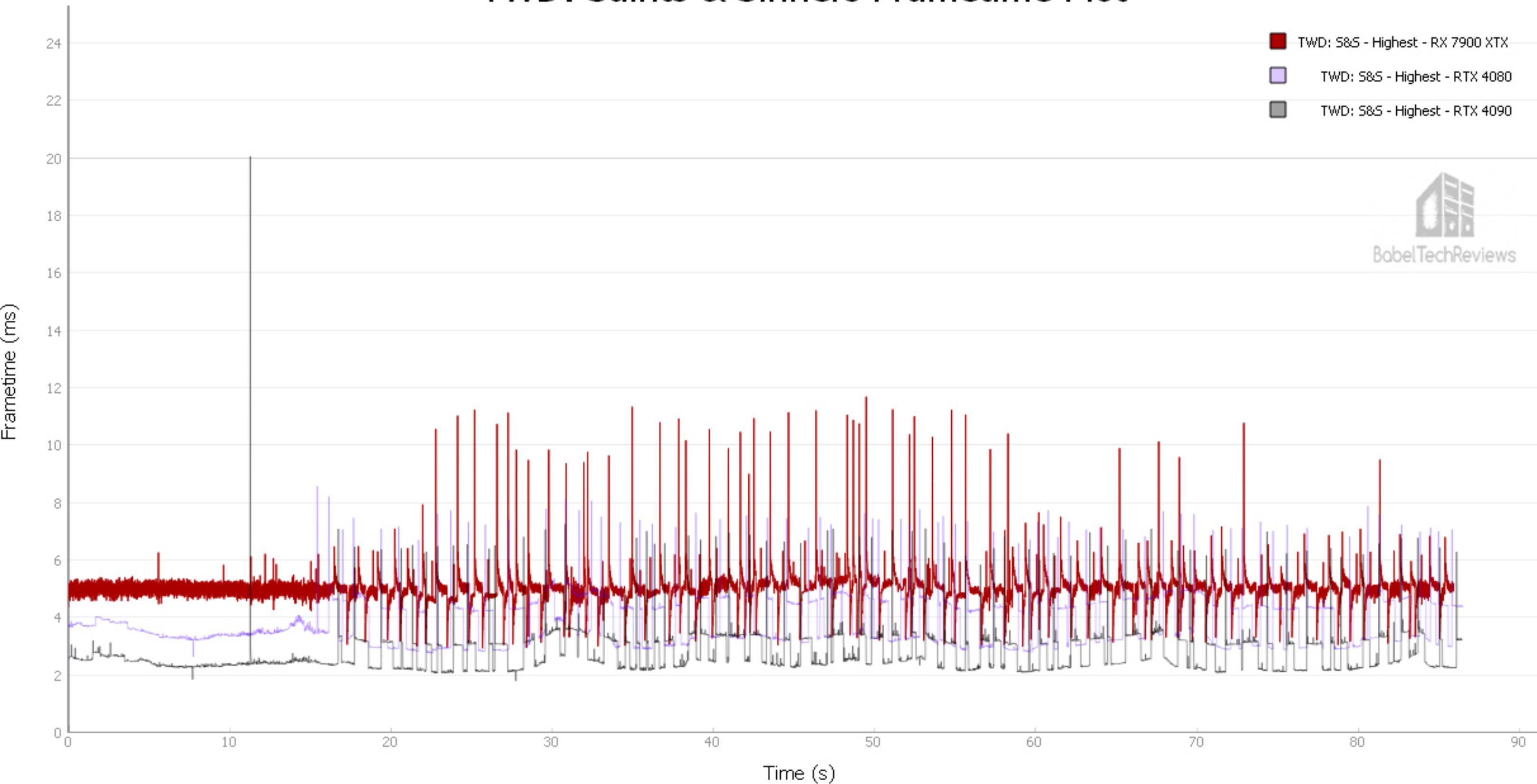
TWD: S&S - Highest - RX 7900 XTX
