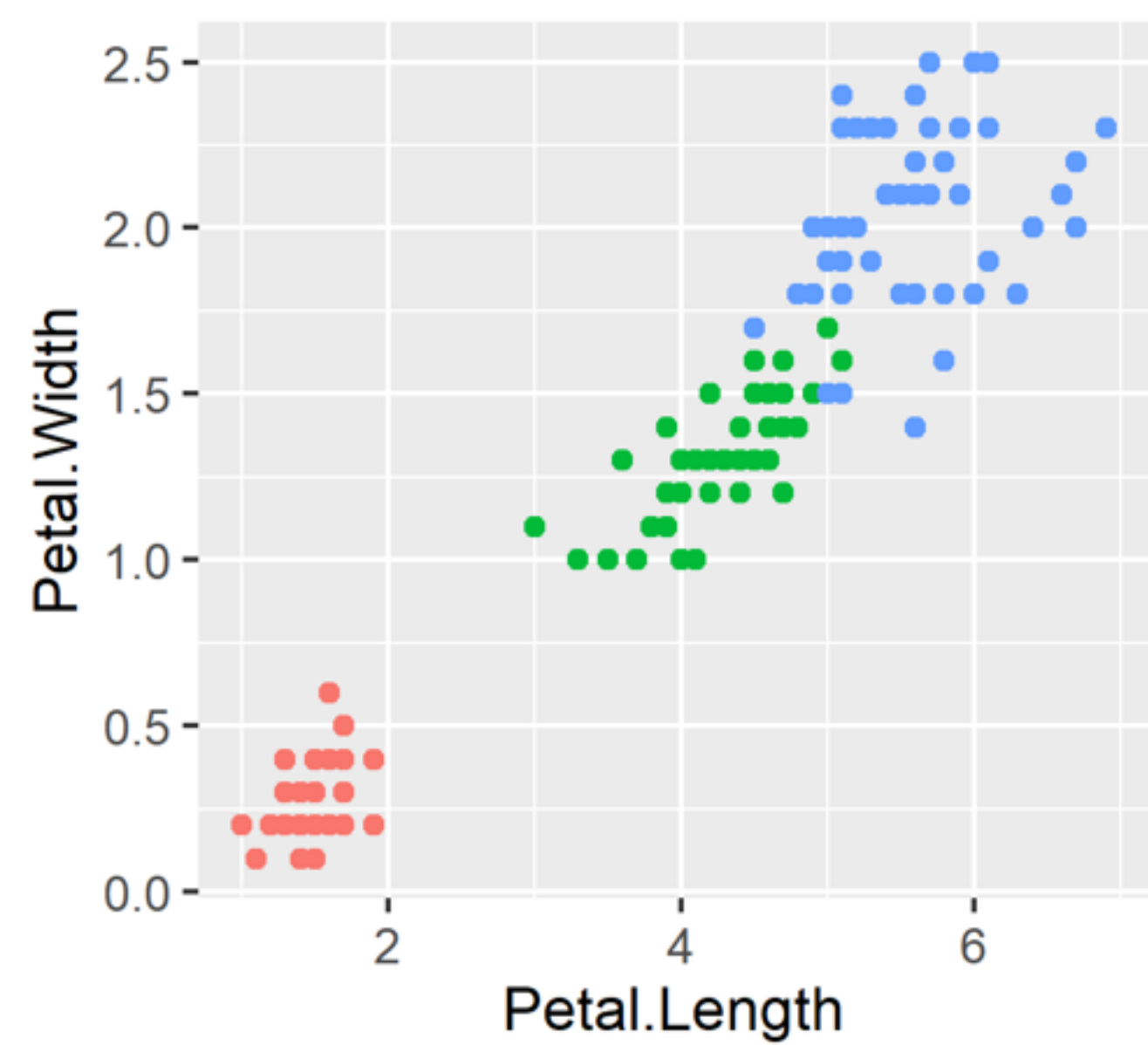
theme_grey()
